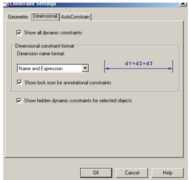
Figure 3: Dimensional constraints
