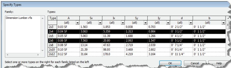
Figure 3: Dimensional lumber family
