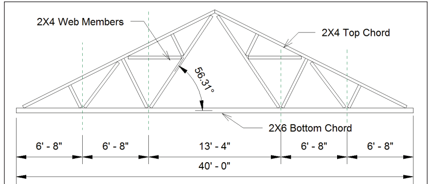
Figure 5: Truss framing elevation
