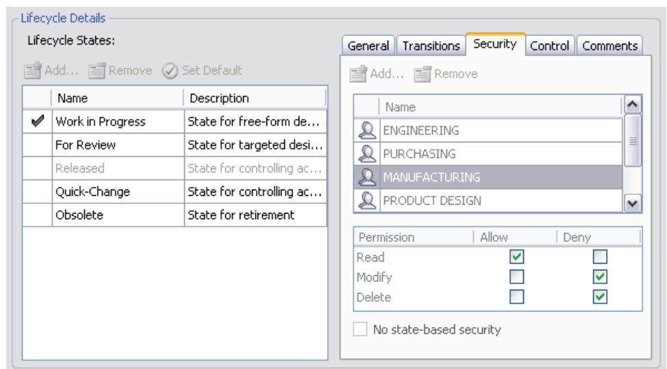
Figure 2: Vault lifecycle security
