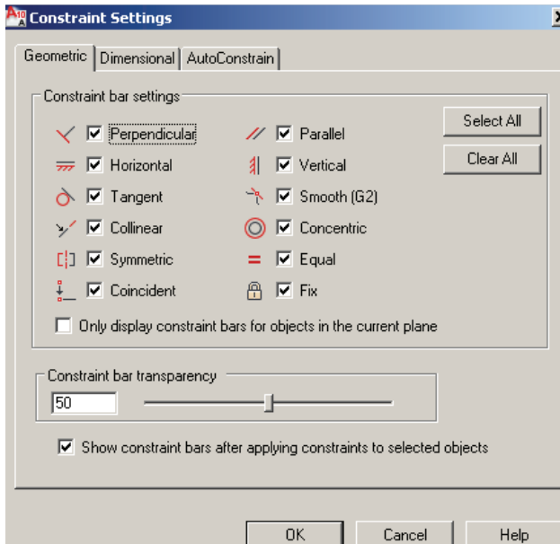
Figure 2: Geometric constraints
