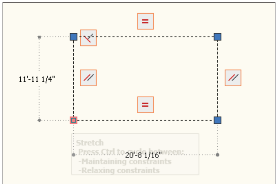
Figure 5: Relaxing constraints
