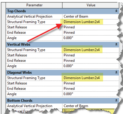
Figure 4: Truss family type properties
