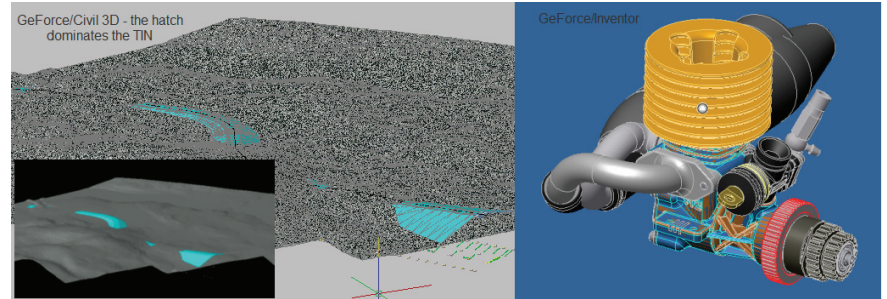
Figure 3: Quadro output
