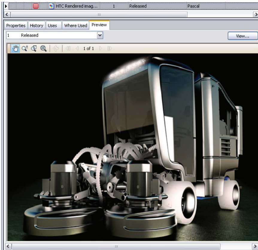
Figure 5: Image viewing
