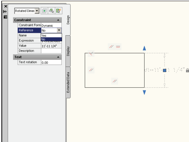
Figure 4: Reference constraints
